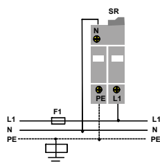
1P + N - Sist. TNS/TT 5SD7 422-2*
