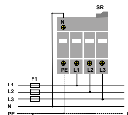
3P + N - Sist. TNS/TT 5SD7 424-4*
