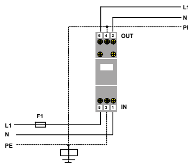
1P + N - Sist. TNS/TT 5SD7 432-2*
